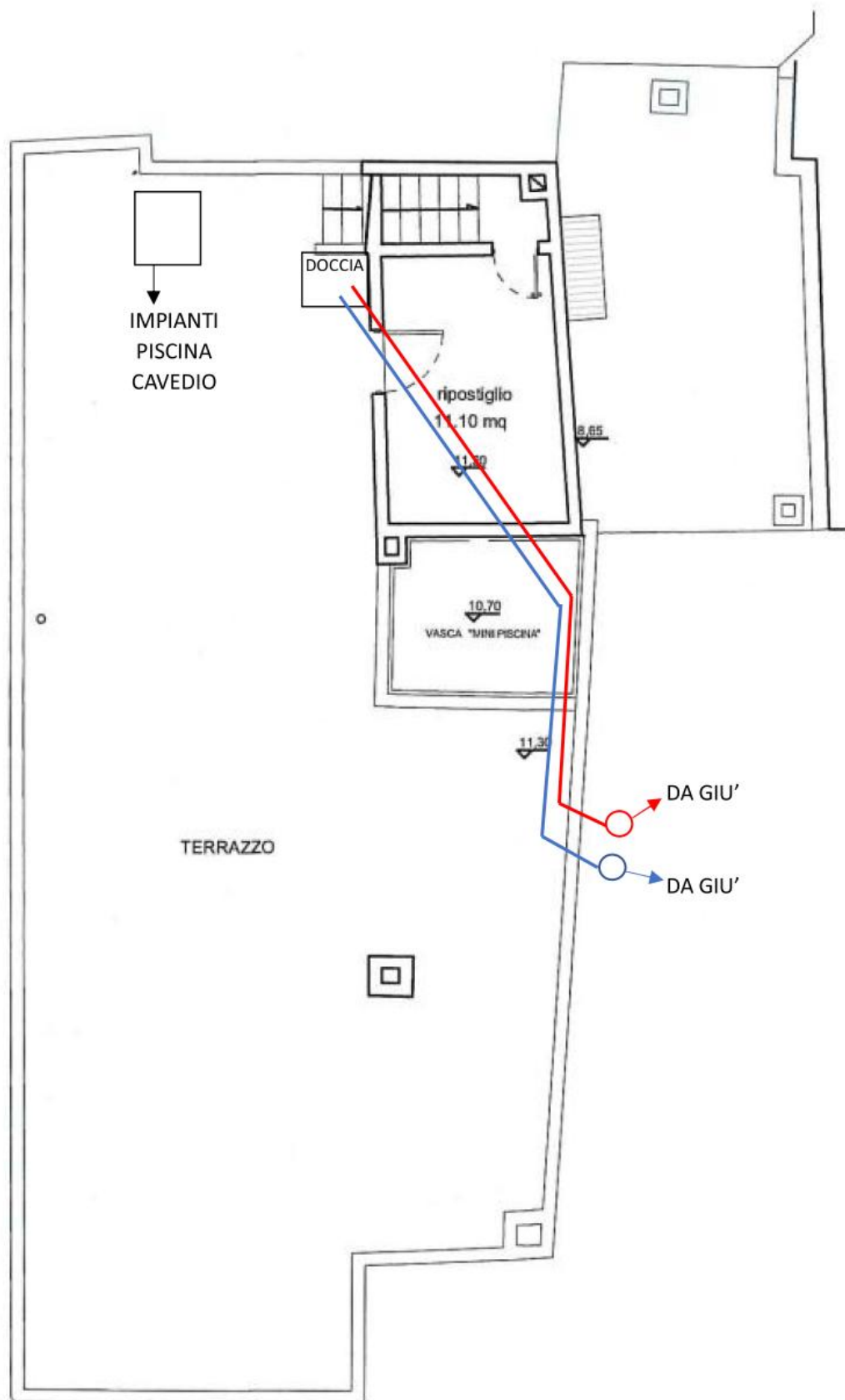
PIANO COPERTURE - scala 1:100
